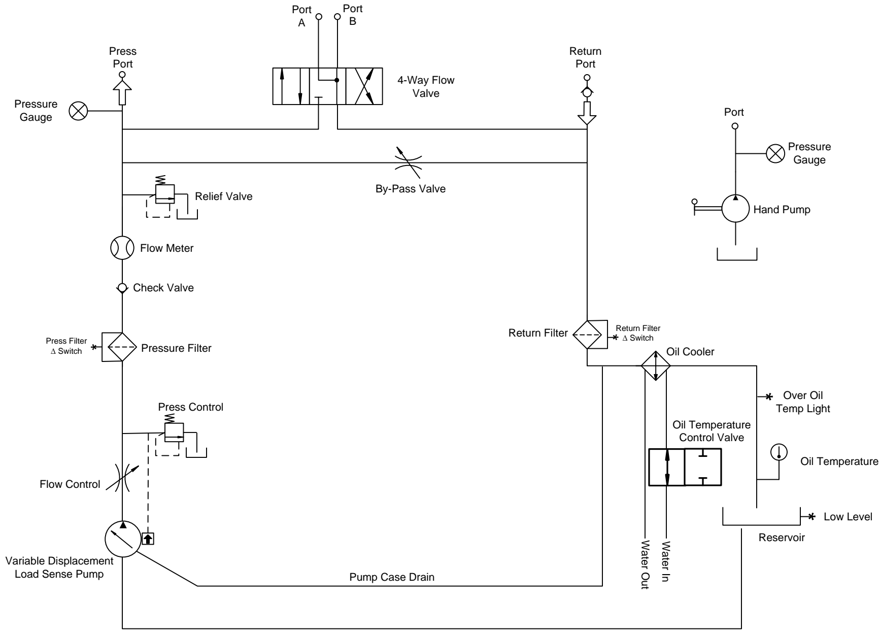
Series 956 Hydraulic Test Stand Schematic
